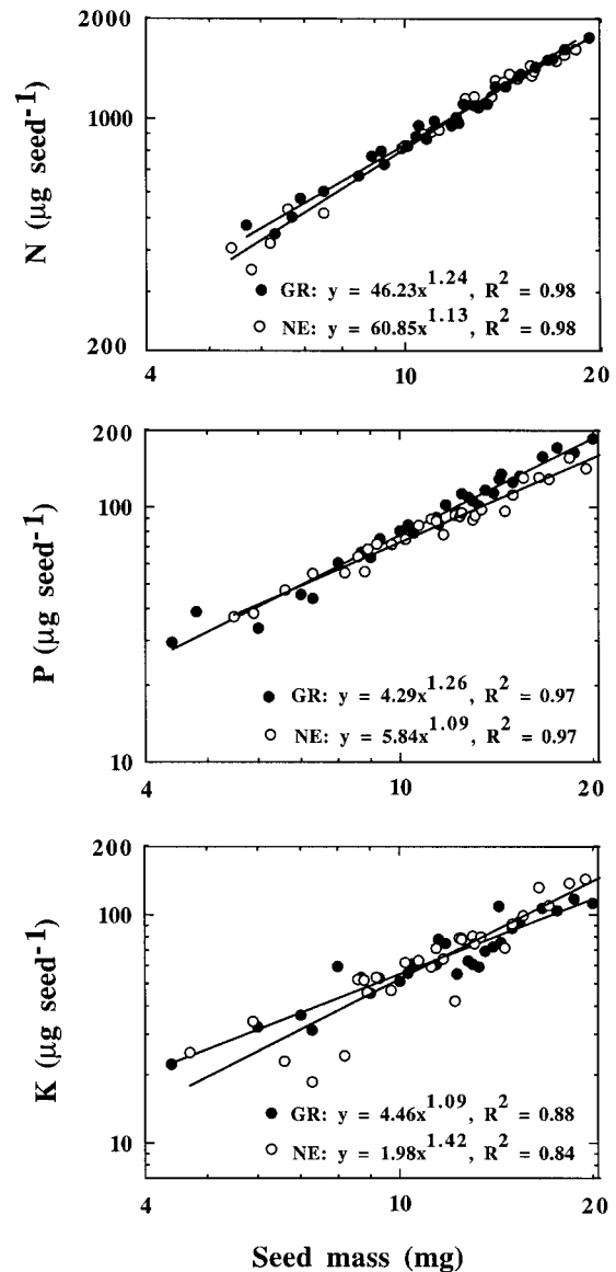
Fig. 1 Relationships between seed mass (mg) and the nitrogen (N), phosphorus (P), and potassium (K) content of seeds ( \mu\text{g seed}^{-1} ) for the Gibraltar Range (GR) and the New England (NE) populations of Banksia cunninghamii . Data are plotted on a log-log scale. For all nutrients, slopes differed significantly between populations. See table 1 for analyses.
