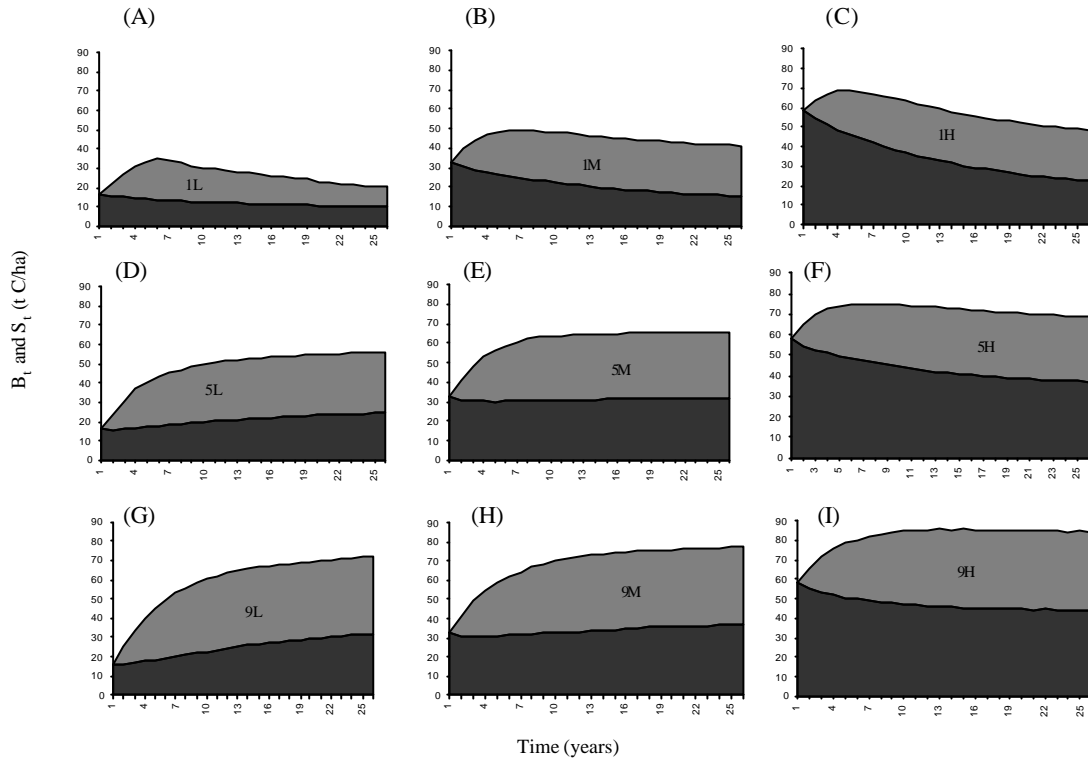
Figure 3. Time-trajectory of above ground (biomass) (light) and soil carbon (dark) stocks under high (C,F,I), medium (B,E,H) and low (A,D,G) initial soil carbon levels.
