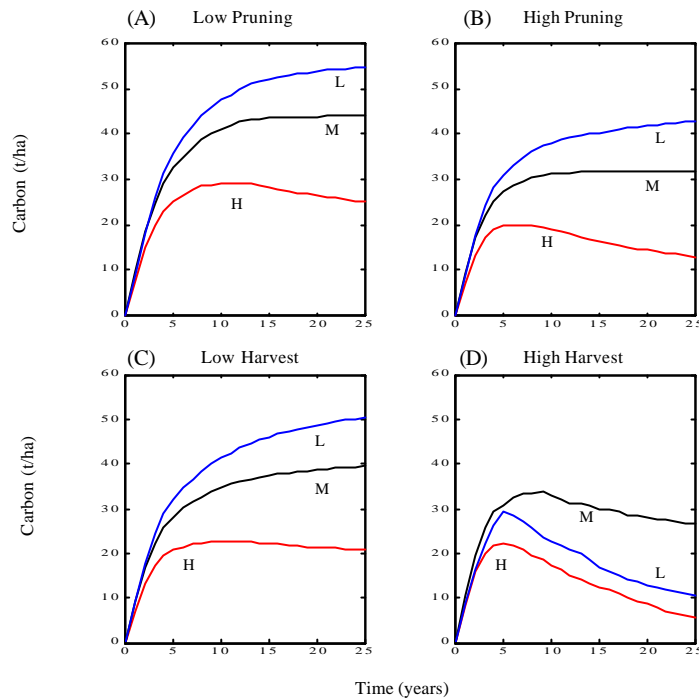
Figure 4: The effect of different initial soil carbon levels on carbon stock (includes soil and standing biomass) relative to baseline, at varying pruning and harvesting levels.
