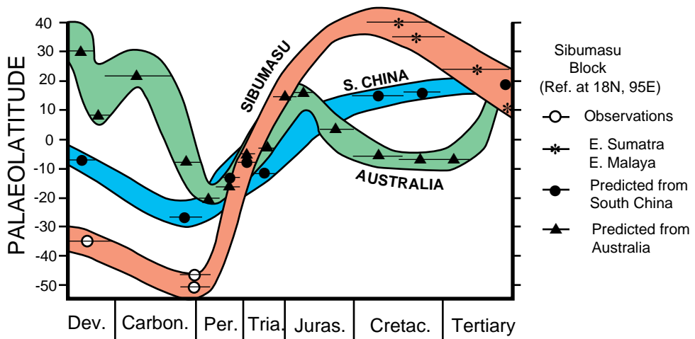
Figure 7. Palaeolatitude versus time plots for the Sibumasu Block (from Van der Voo, 1993).
