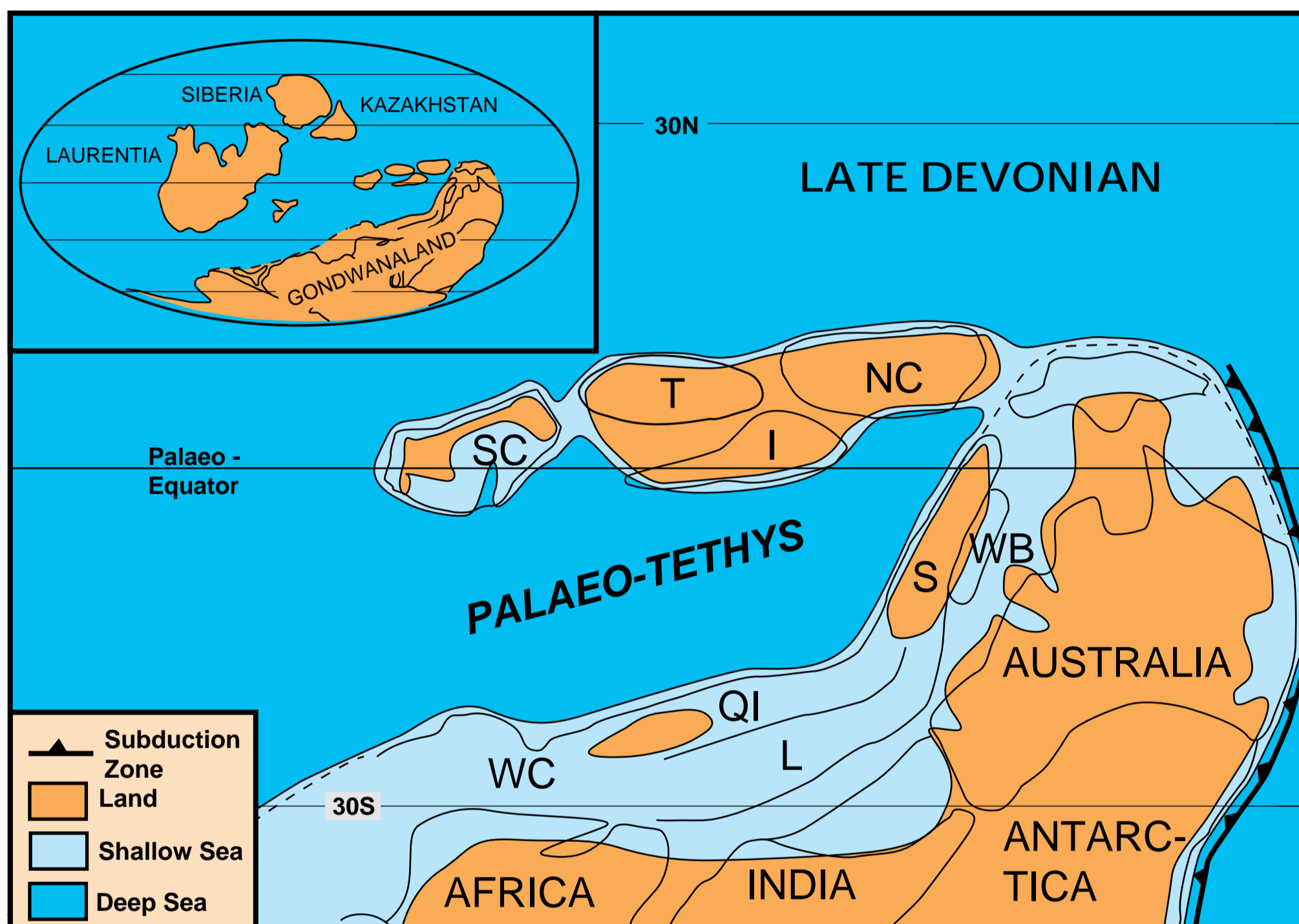
Figure 3. Reconstruction of eastern Gondwanaland for the Late Devonian showing the postulated positions of the East and Southeast Asian terranes, distribution of land and sea, and opening of the Palaeo-Tethys ocean at this time. Present day outlines are for reference only. Distribution of land and sea for Chinese blocks principally from Wang (1985). Land and sea distribution for Pangea/Gondwanaland compiled from Golongka et al. (1994), Smith et al. (1994); and for Australia from Struckmeyer & Totterdell (1990). NC = North China SC = South China T = Tarim I = Indochina Qi = Qiangtang L = Lhasa S = Sibumasu WC = Western Cimmerian Continent WB = West Burma.
