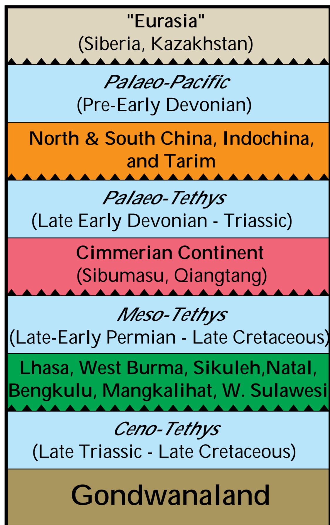
Figure 2. Schematic diagram showing the three continental slivers/collages of terranes, rifted from Gondwanaland and translated northwards by the opening and closing of the three successive Tethyan oceans, the Palaeo-Tethys, Meso-Tethys and Ceno-Tethys.
